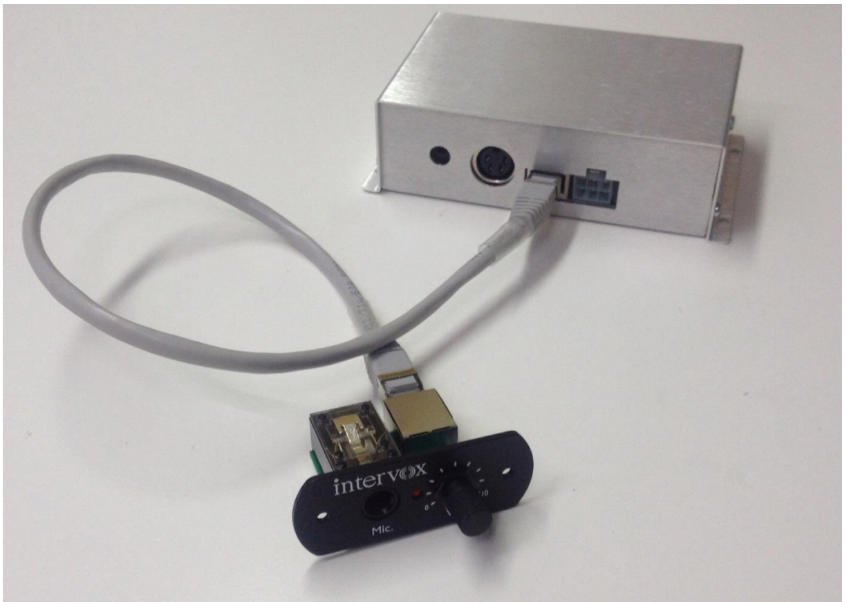
Command Unit with Remote Control Connector
